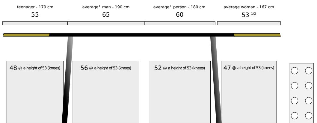
VIENNA-MILANO-AMSTERDAM-LISBOA-MADRID extended for 8 p. in 2:2:2:2 arrangement extended with plug-in end extensions extended desktop 235 cm
