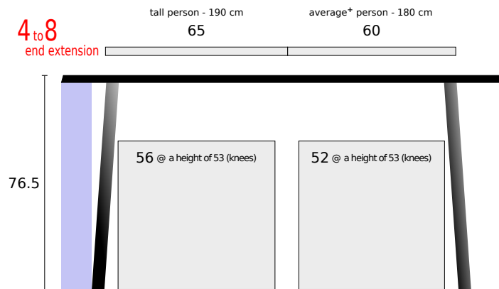
VIENNA-MILANO-AMSTERDAM-LISBOA-MADRID dining table for 4 p. in 2:2 arrangement extendible with plug-in end extensions desktop 157 cm
