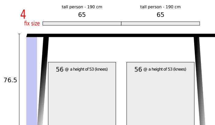
VIENNA-MILANO-AMSTERDAM-LISBOA-MADRID dining table for 4 p. in 2:2 arrangement not extendible desktop 157 cm
